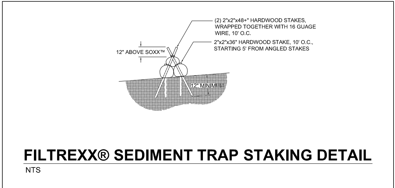
Figure 9.2. Engineer Design Detail for Staking Sediment Trap.
